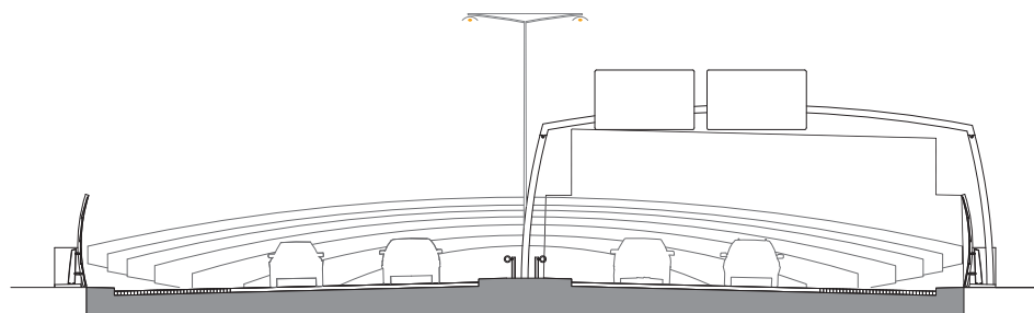
Snit C 1:200
